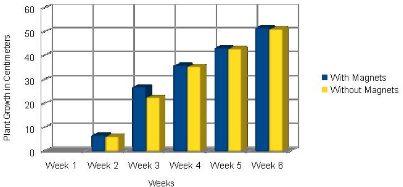
Plant Growth With and Without Magnets
